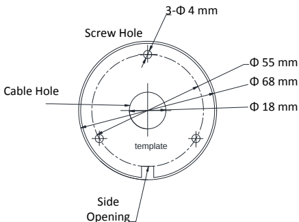
Figure 2-2 The Drill Template
