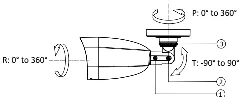
Figure 2-4 3-axis Adjustment
