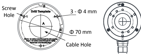
Figure 2-5 The Drill Template
