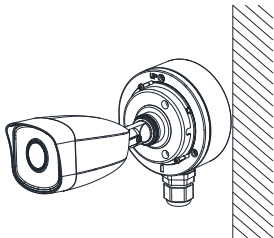
Figure 2-8 Combine Junction Box's Cover with its Body
