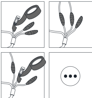
Figure 2-10 Waterproof Cables
